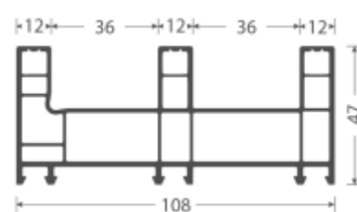
Sliding 3 Track Outer Frame AP-12
