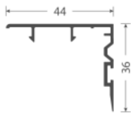
Sliding Interlock for 66 & 80 mm Sash
