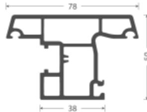
Casement Window Sash-Grill option AP-04
