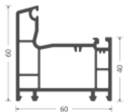
Casement Outer Frame AP-01
