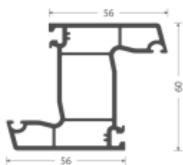
Casement Z Mullian AP-07
