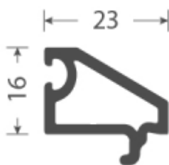
Glazing Bead 23 mm
