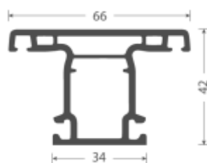
Sliding T Mullian for 66 & 80 mm Sash
