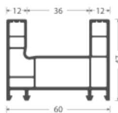
Sliding 2 Track Outer Frame AP-11
