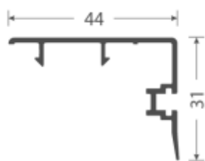
Sliding Interlock for 56 mm sash
