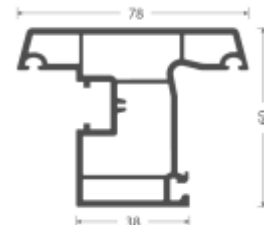
Casement Window Sash AP-05
