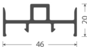
Multipane Adaptor for 66 & 80 mm Sash
