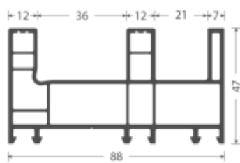
Sliding 2.5 Track Outer Frame AP-13
