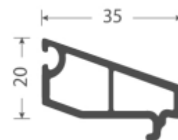
Glazing Bead 35 mm
