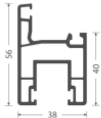
Sliding Sash 56 mm AP-15
