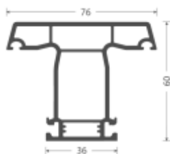
Casement T Mullian AP-03
